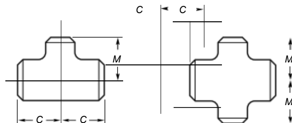
DIMENSIONS OF REDUCING OUTLET TEES AND REDUCING OUTLET CROSSES
